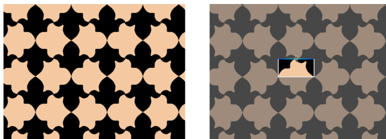
Figure 10: (left) A pattern from Alhambra with reflections and 2-gyration centers; (right) a minimal region
