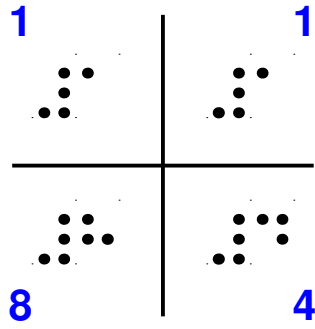
Atractor J24 – 1.7.14
