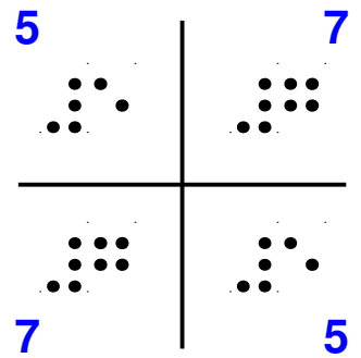
Atractor J24 – 1.7.24
