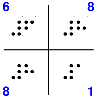
Atractor J24 – 1.7.20
