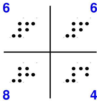
Atractor J24 – 1.7.23
