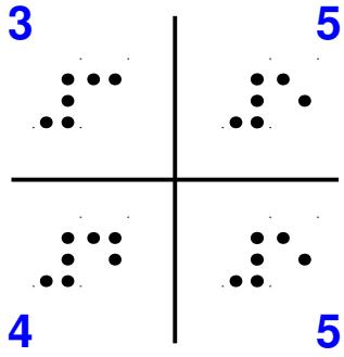
Atractor J24 – 1.7.13
