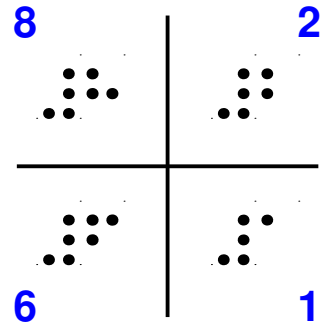
Atractor J24 – 1.7.18
