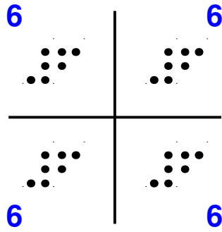
Atractor J24 – 1.7.17
