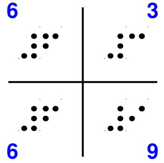
Atractor J24 – 1.7.15
