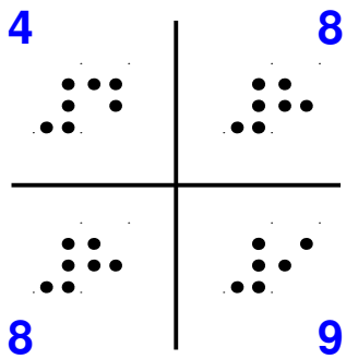
Atractor J24 – 1.7.22
