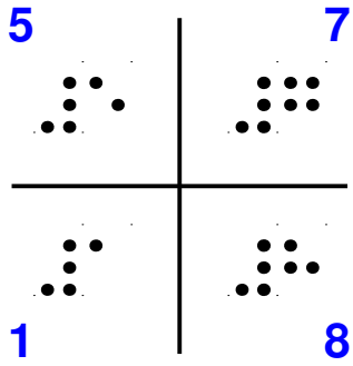
Atractor J24 – 1.7.19
