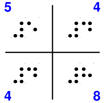
Atractor J24 – 1.7.21
