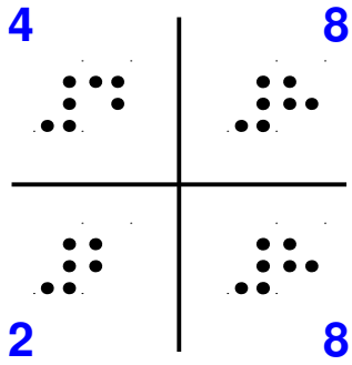
Atractor J24 – 1.7.16
